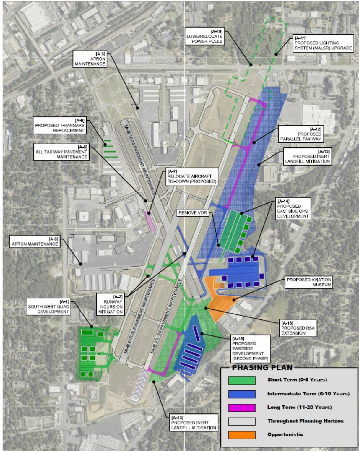
Figure 1-3: Proposed Airside Projects
