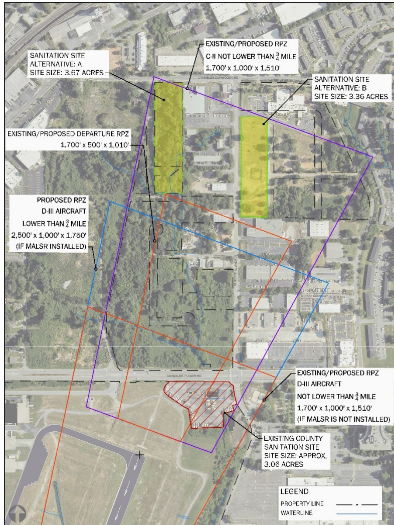
Figure 5-3: North RPZ Protentional Developable Land
