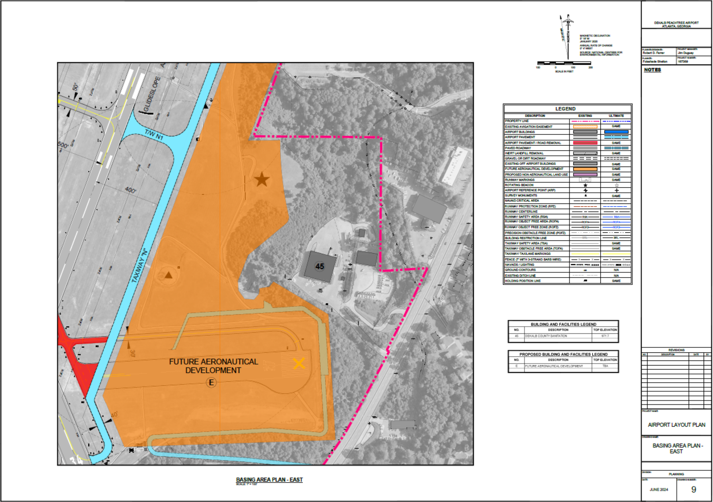
Figure 6-9: Basing Area Plan - East
