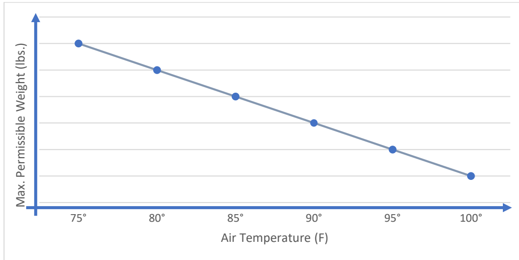
Figure 4-5: Aircraft Weight vs. Air Temperature
