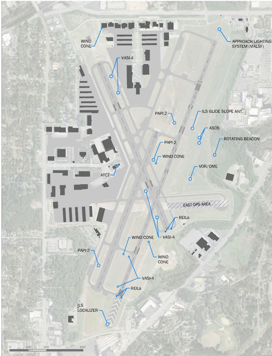
Figure 2-3: NAVAIDs
