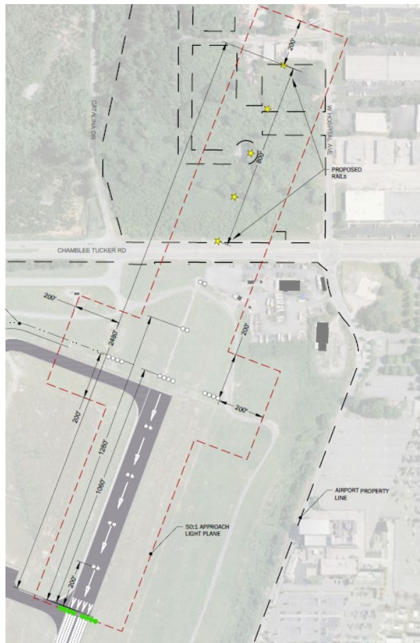
Figure 5-1: Upgrade Approach Lights to MALSR
