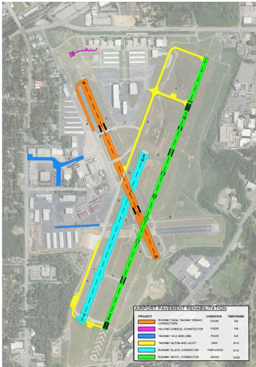
Figure 7-3: Airfield Pavement Rehabilitation Phasing
