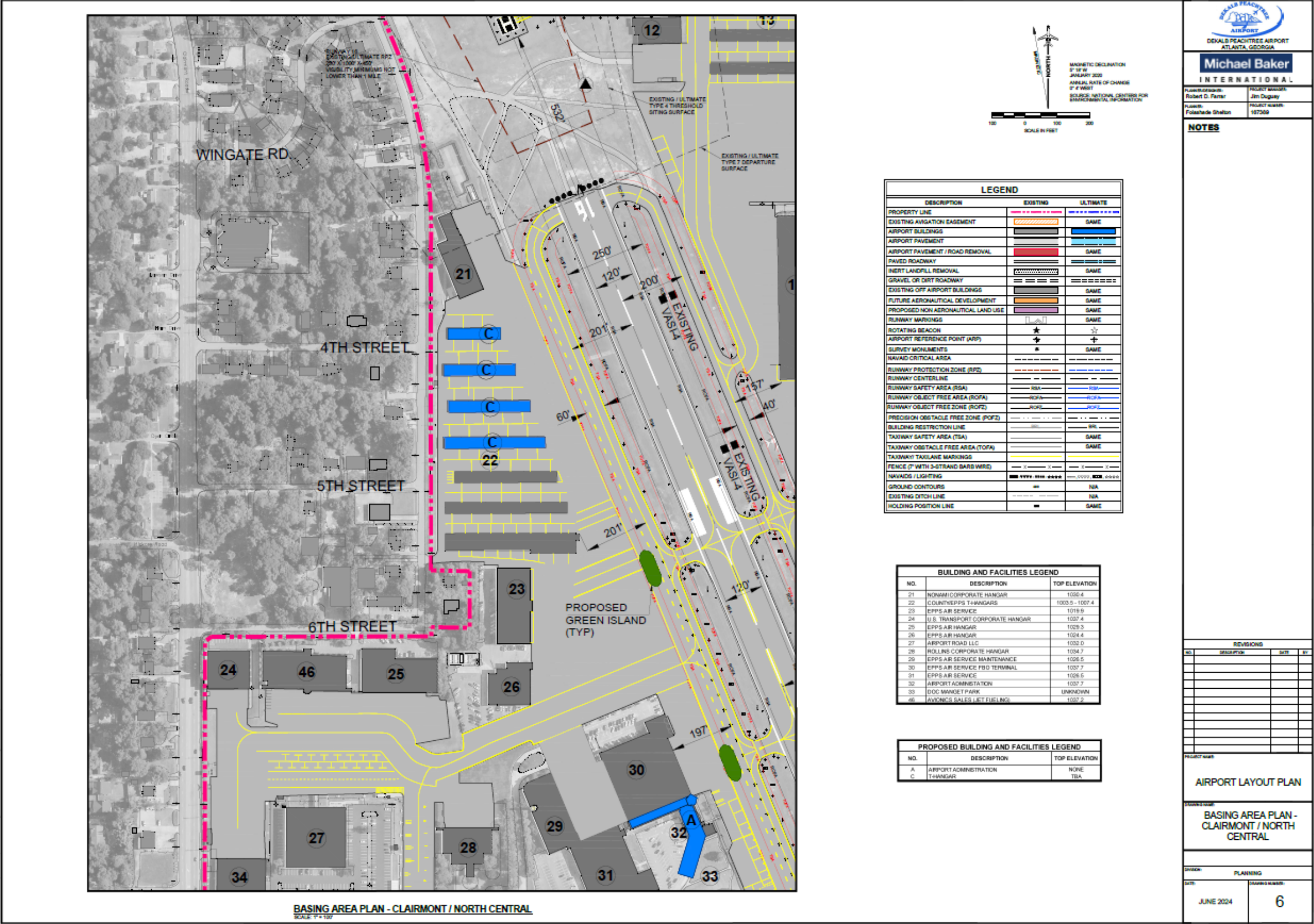
Figure 6-6: Basing Area Plan – Clairmont/North Central
