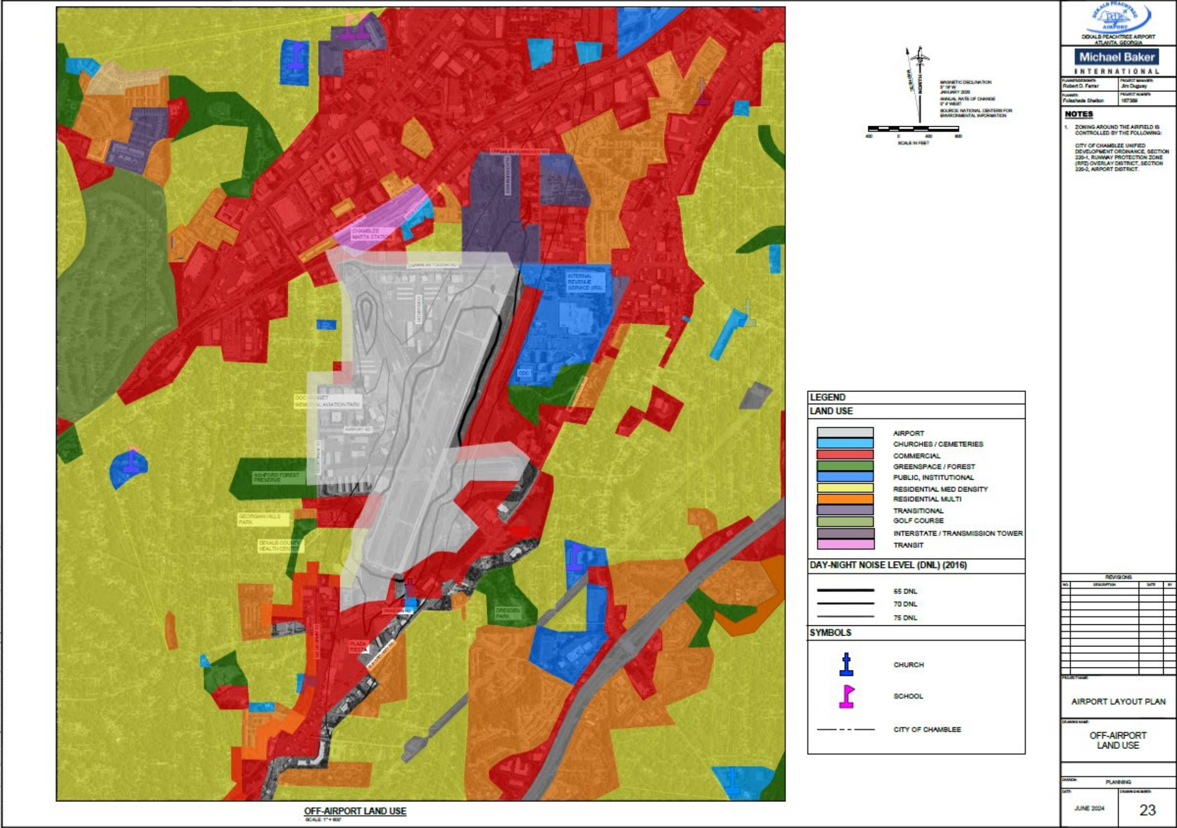
Figure 6-23: Off-Airport Land Use
