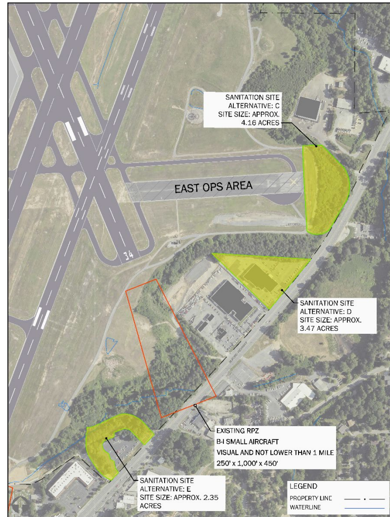
Figure 5-4: North RPZ Protentional Developable Land
