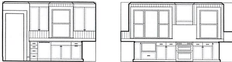
3 EXISTING KITCHEN WINDOW SASHES SCALE: 1/4" = 1'-0"
