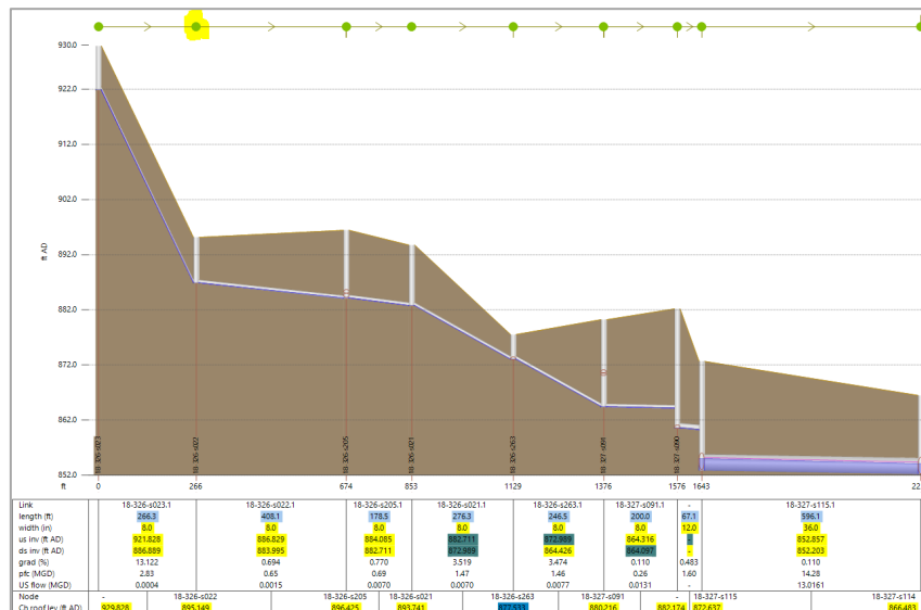
Hydraulic Model Profile for MH 18-326-s022
