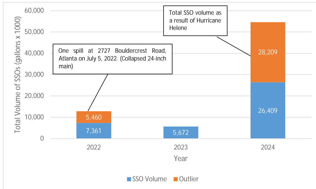
Figure ES-3 Reported Volumes of SSOs by Year (2022–2024)
