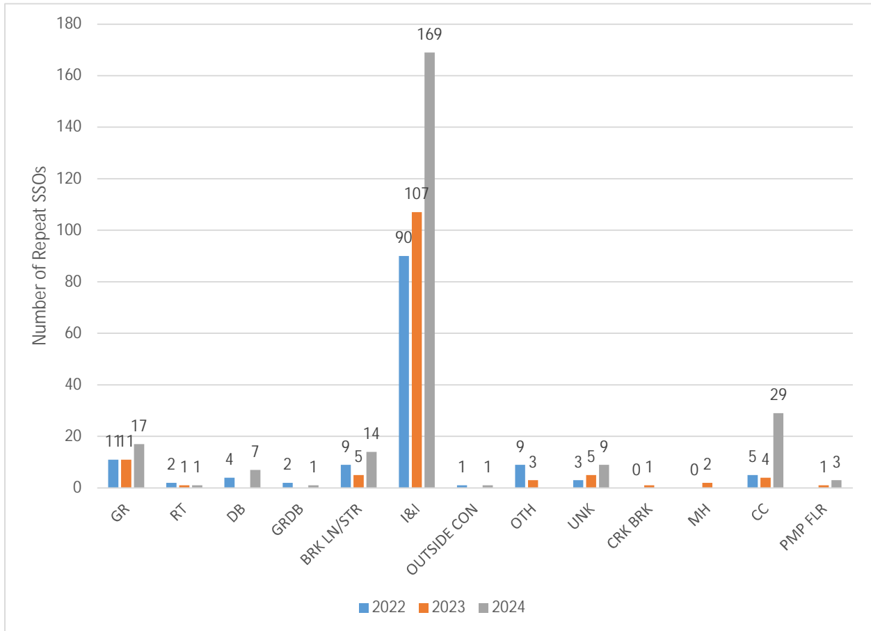
Figure 5-6 Number of Repeat SSOs by Cause (2022–2024)
