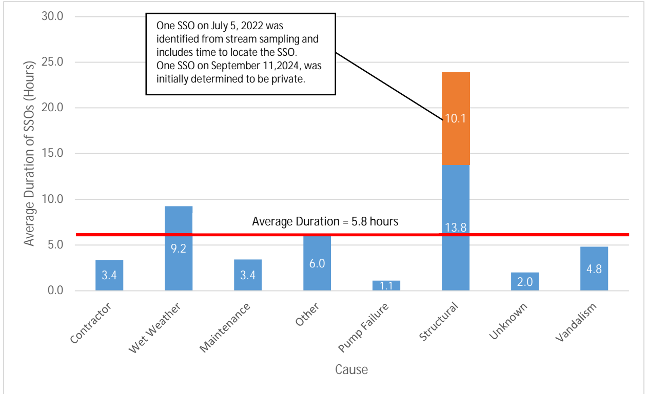
Figure 3-2 Average SSO Duration by Cause (2022–2024)
