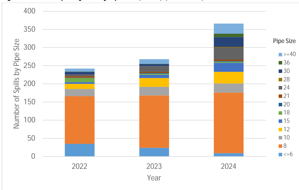
Figure 5-2 Spills by Year by Pipe Size (Inches) (2022–2024)
