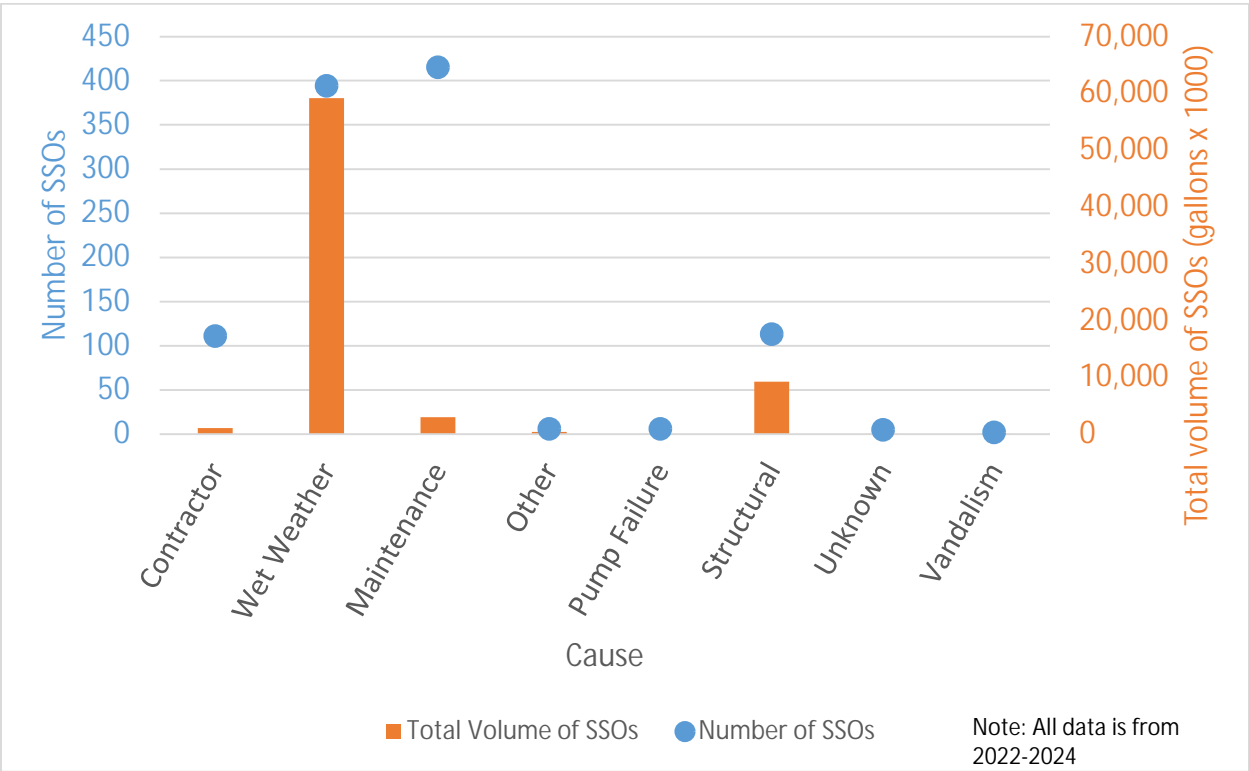
Figure 4-1 SSOs by Count, Volume, and Cause (2022–2024)
