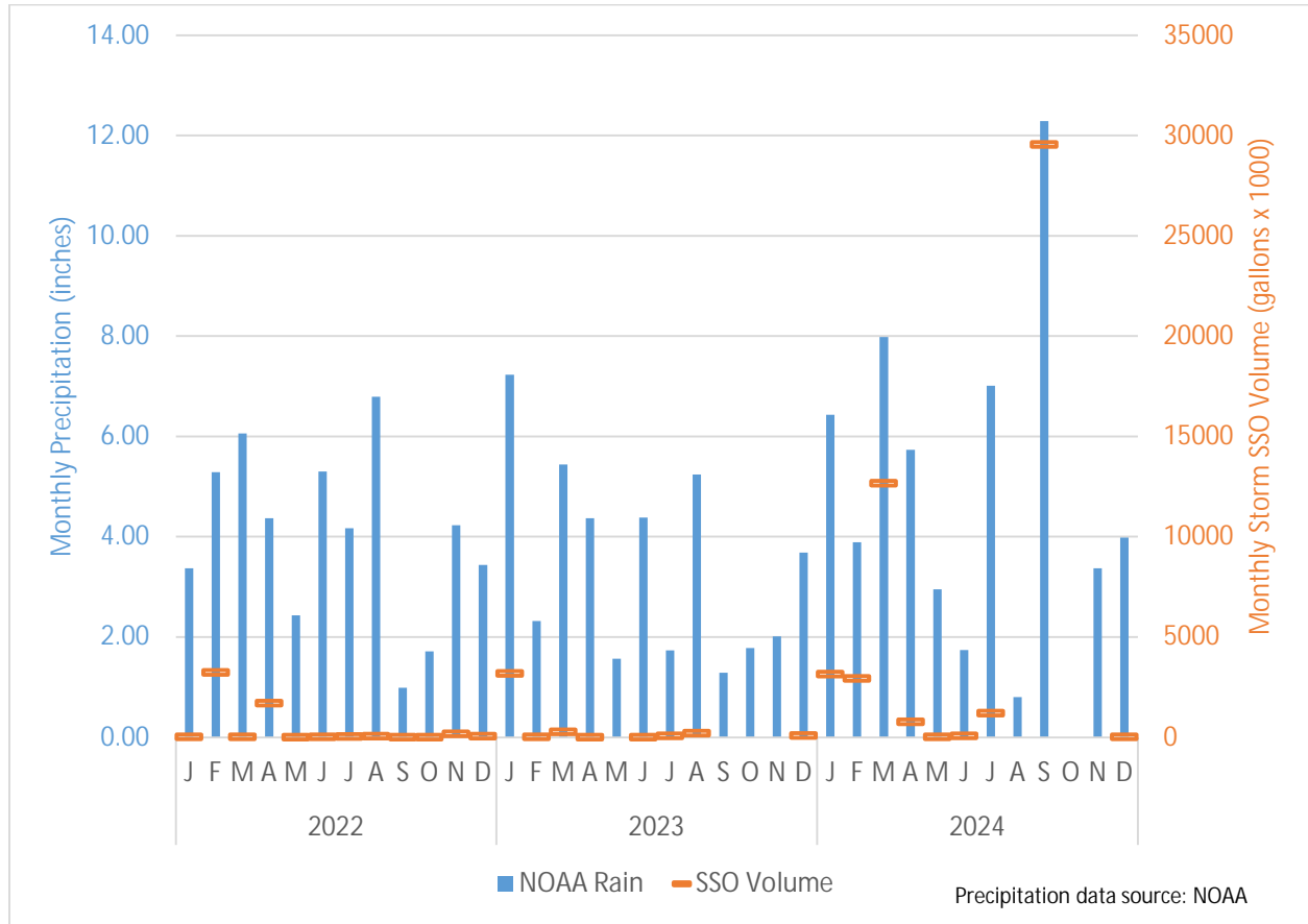
Figure 5-4 Monthly Precipitation and Wet-Weather-Induced SSO Volume (2022–2024)
