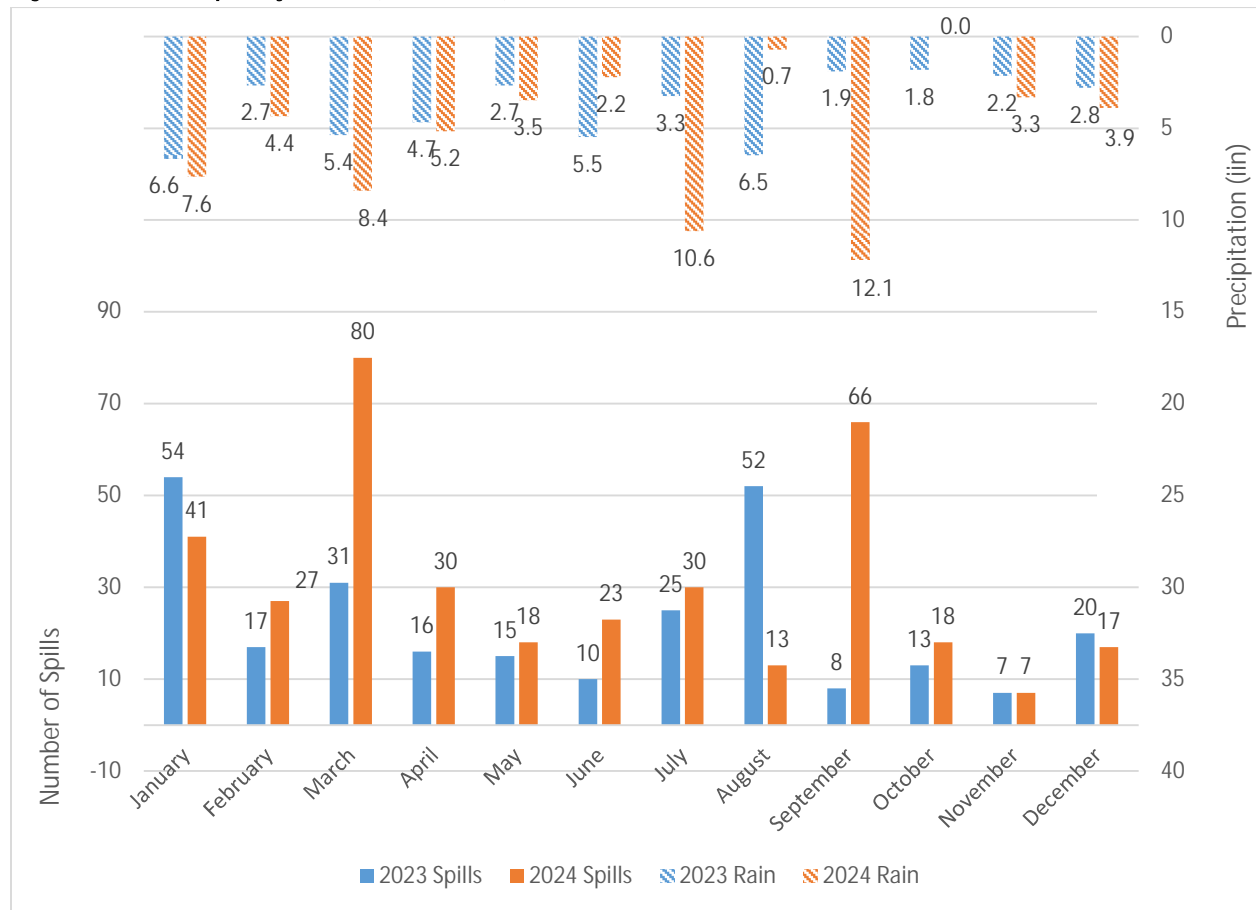
Figure 4-5 Spills by Month (2023–2024)
