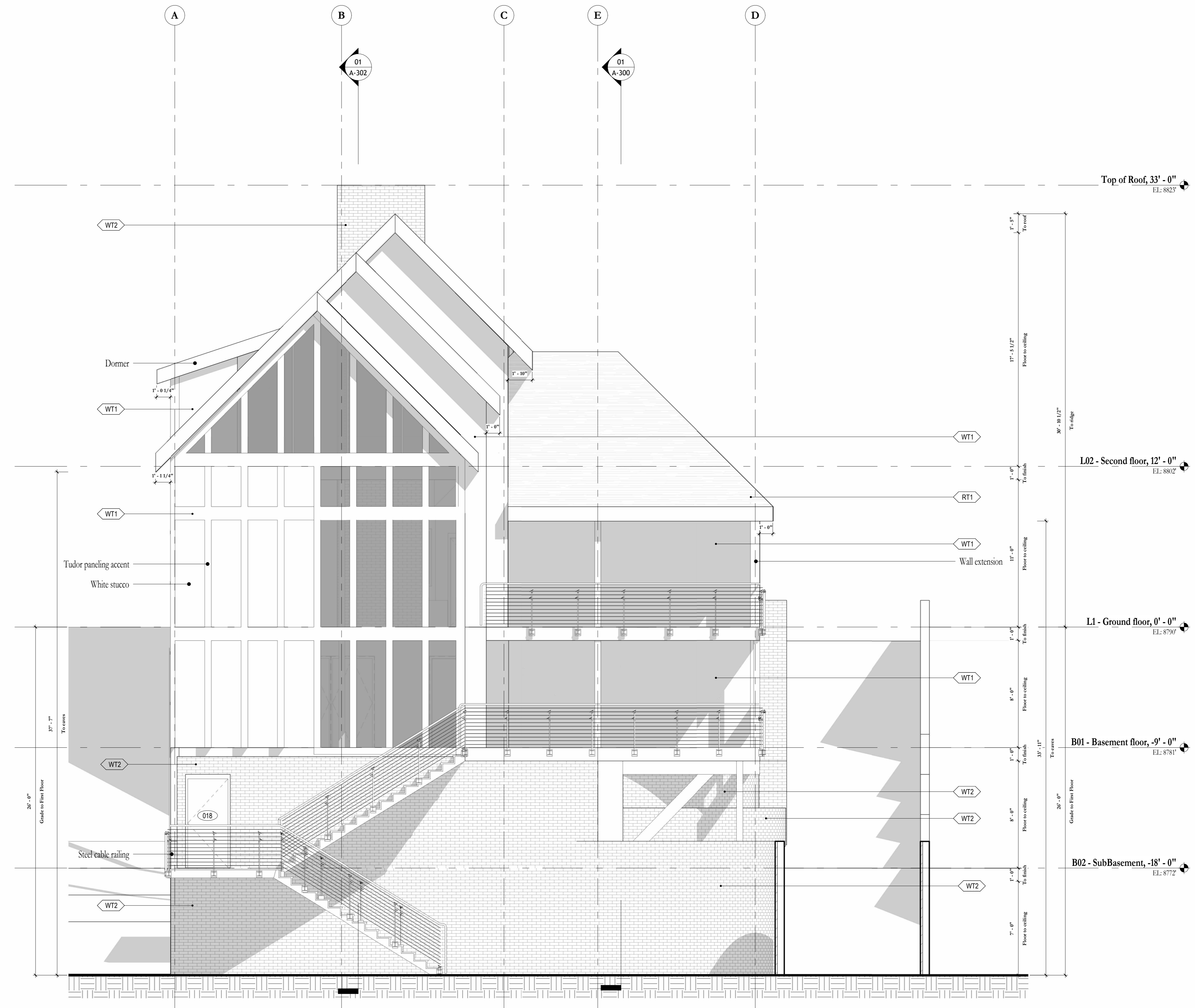
01 North Architectural Building Elevation A-200 1/4" = 1'-0"
