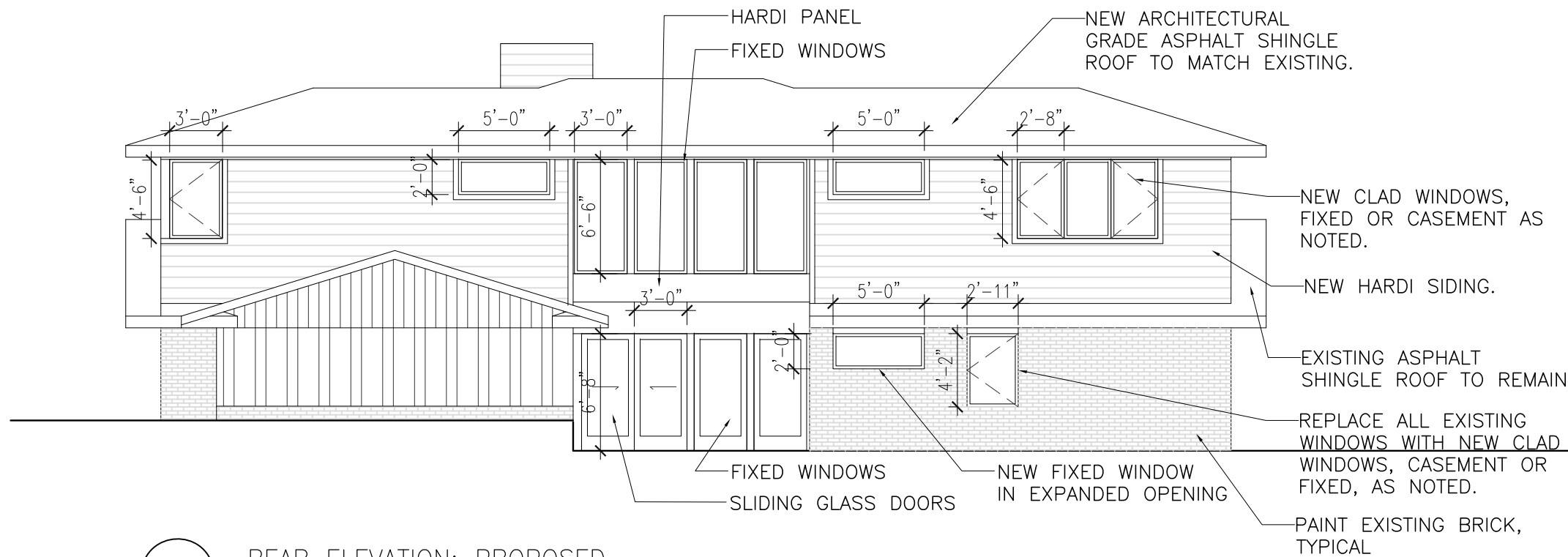
02 REAR ELEVATION: PROPOSED SCALE: 1/8" = 1'-0"
