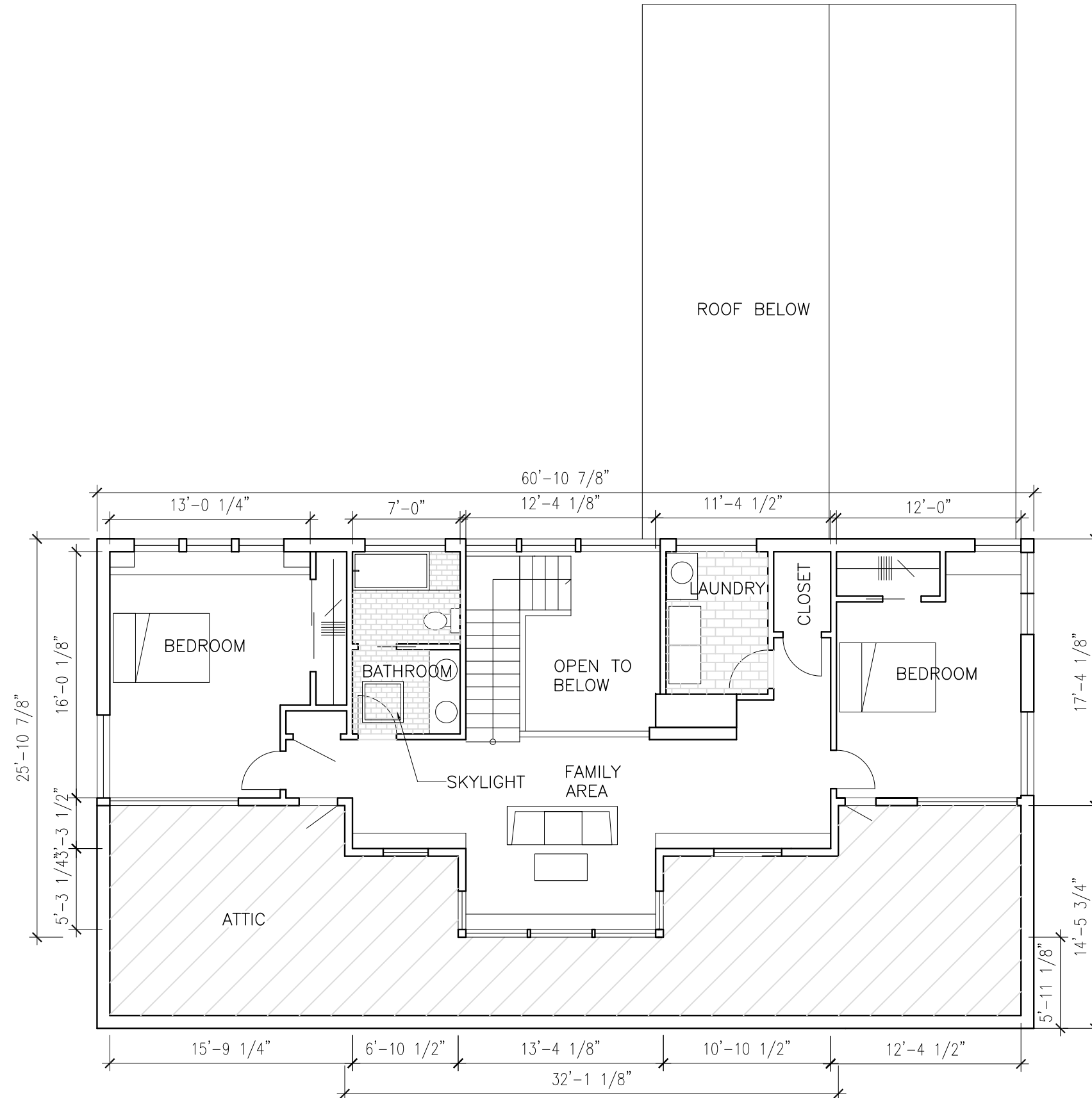
01 SECOND FLOOR PLAN, PROPOSED SCALE: 1/8" = 1'-0"
