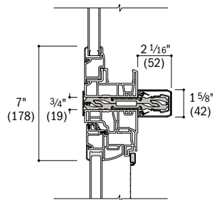
Twin Transom Over Twin Awning
