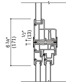
Picture/Single Transom/Specialty Over Gliding
