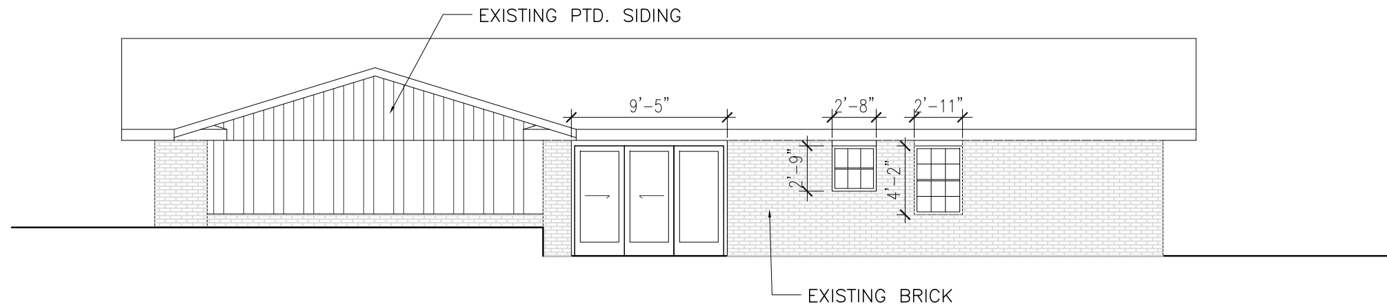
01 REAR ELEVATION: EXISTING SCALE: 1/8" = 1'-0"
