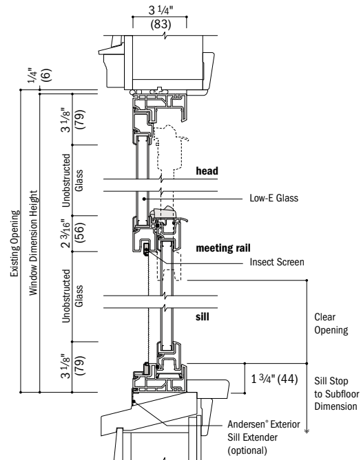
Vertical Section
