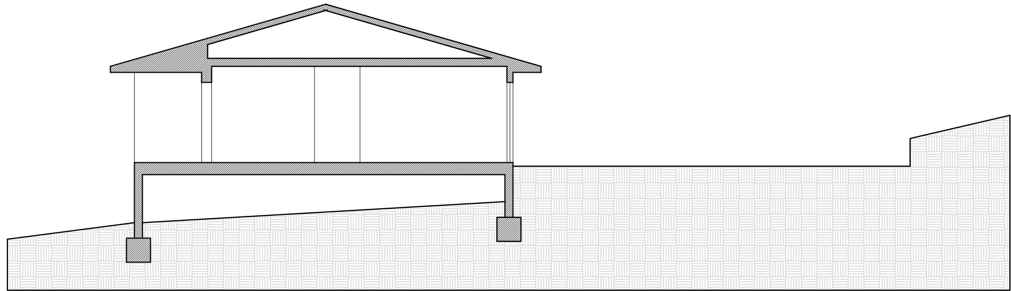
01 BUILDING SECTION, EXISTING SCALE: 1/8" = 1'-0"
