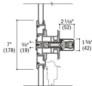
Twin Transom Over Twin Single-Hung
