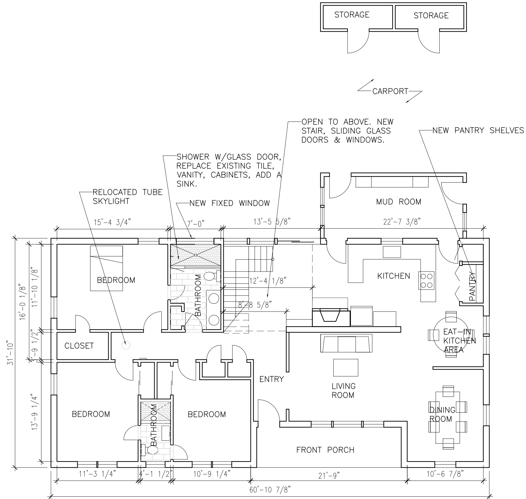
01 FIRST FLOOR PLAN, PROPOSED SCALE: 1/8" = 1'-0"
