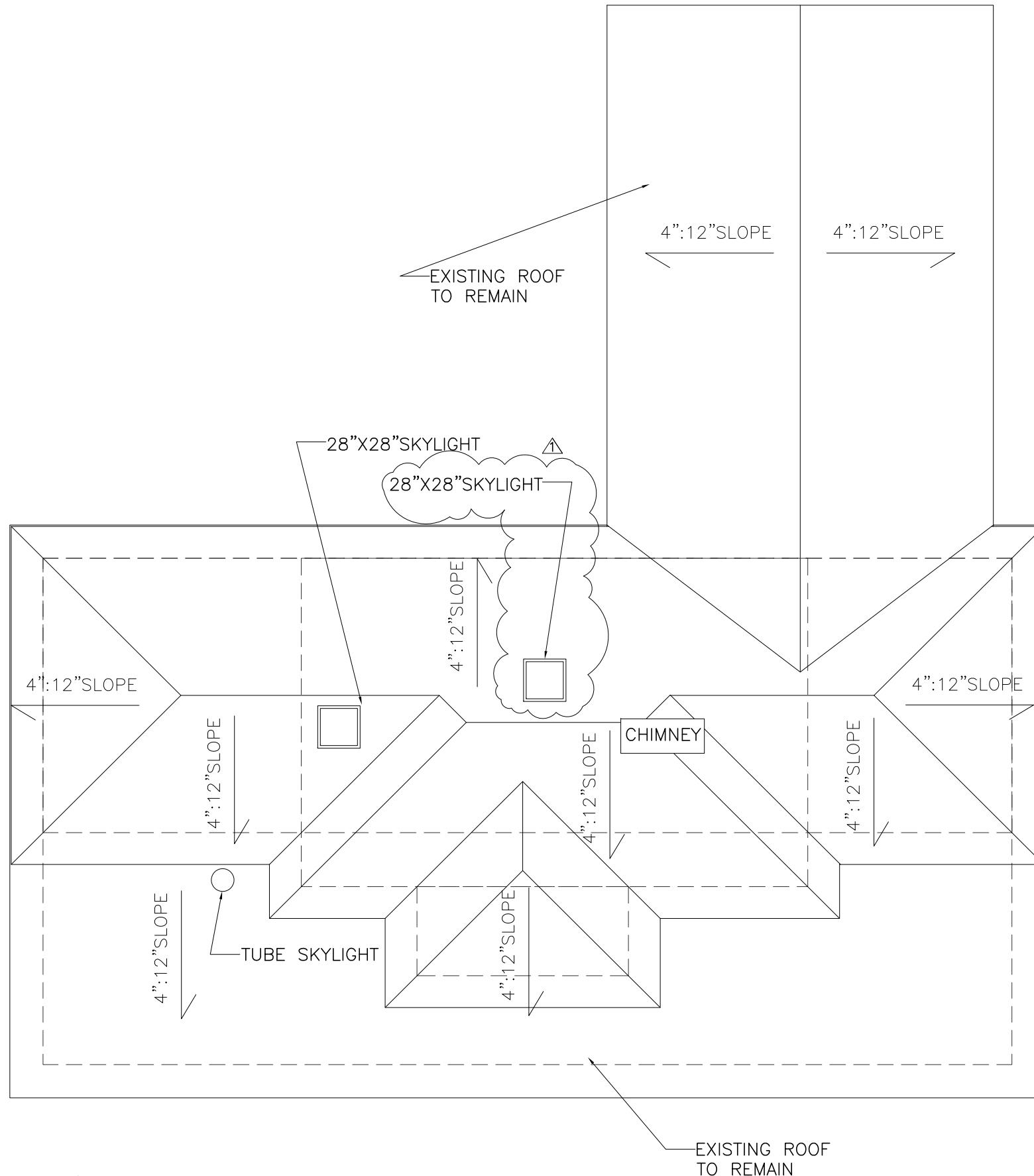
01 ROOF PLAN: PROPOSED SCALE: 1/8" = 1'-0"
