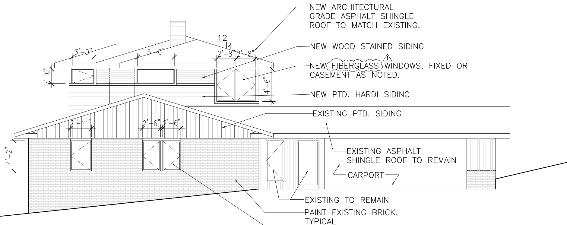
02 SIDE ELEVATION, DRIVEWAY: PROPOSED SCALE: 1/8" = 1'-0"
