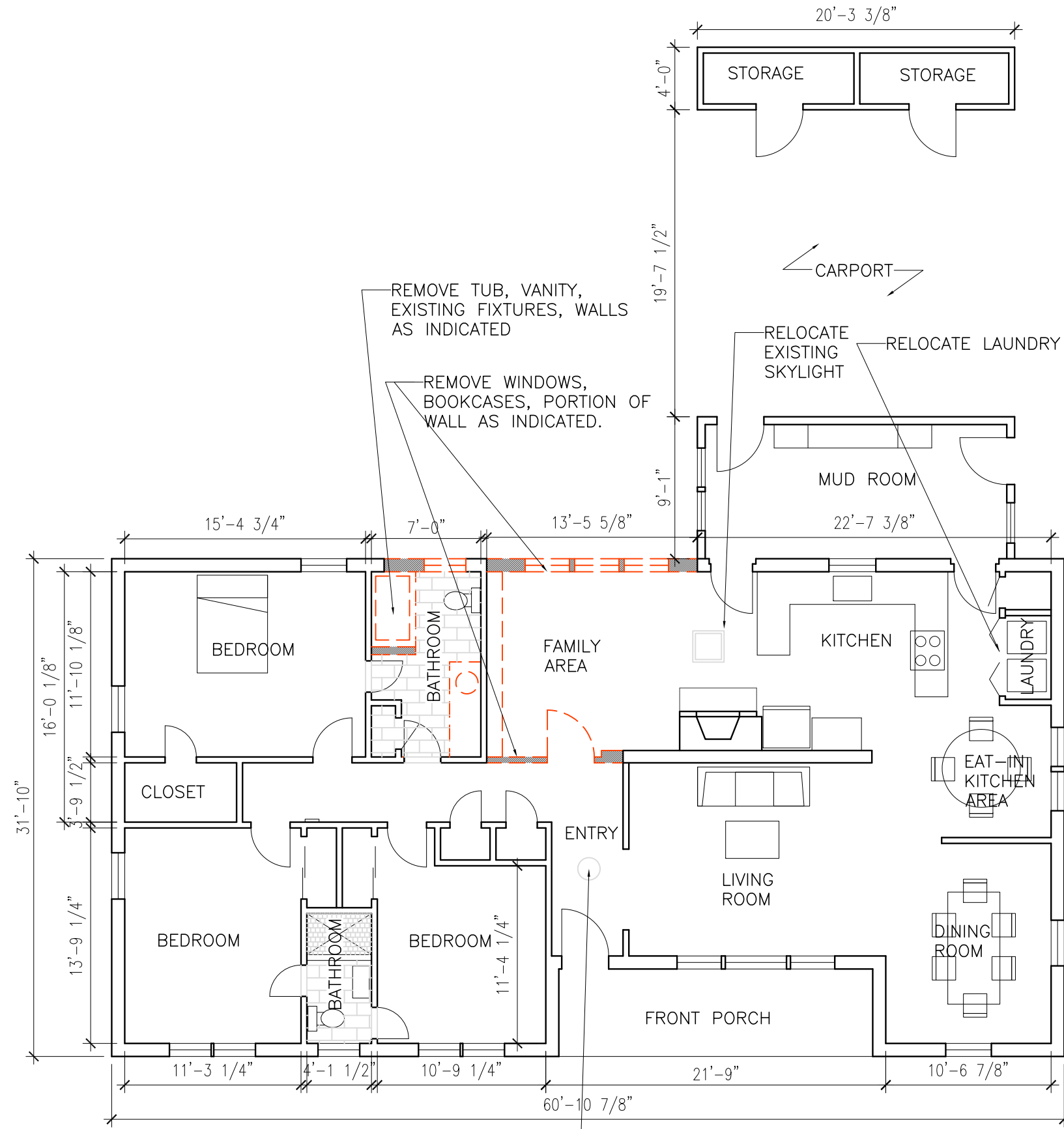
01 FIRST FLOOR PLAN, EXISTING SCALE: 1/8" = 1'-0"
