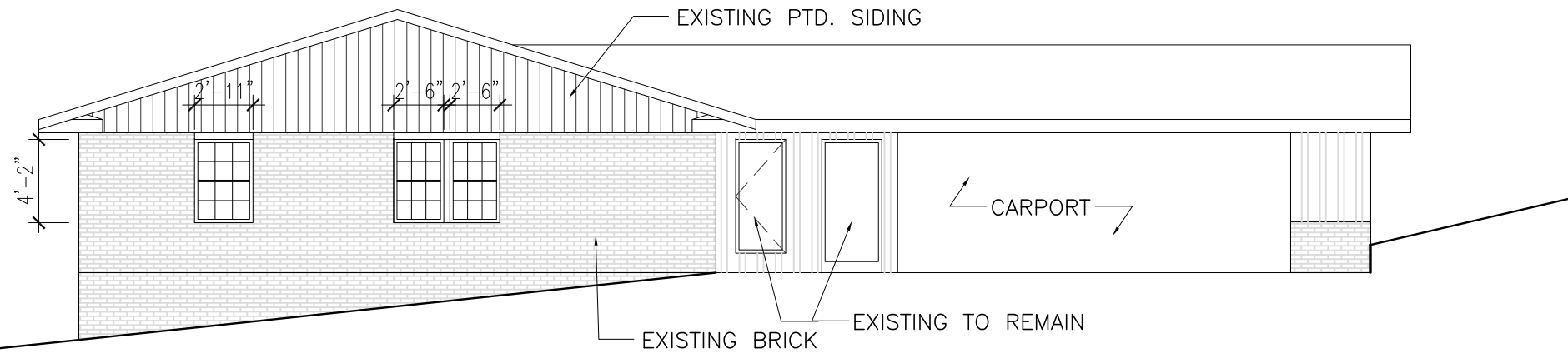
01 SIDE ELEVATION, DRIVEWAY: EXISTING SCALE: 1/8" = 1'-0"
