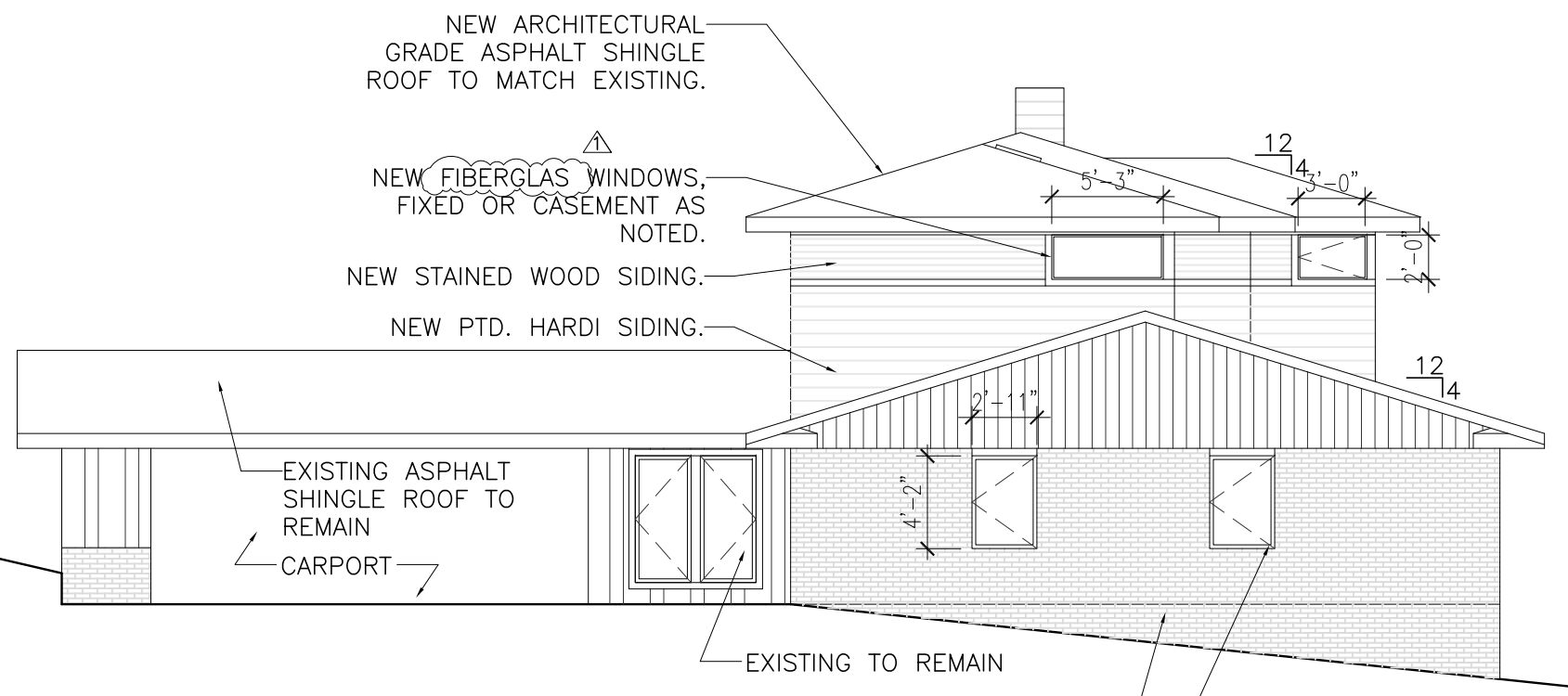
02 SIDE (EAST) ELEVATION: PROPOSED SCALE: 1/8" = 1'-0"
